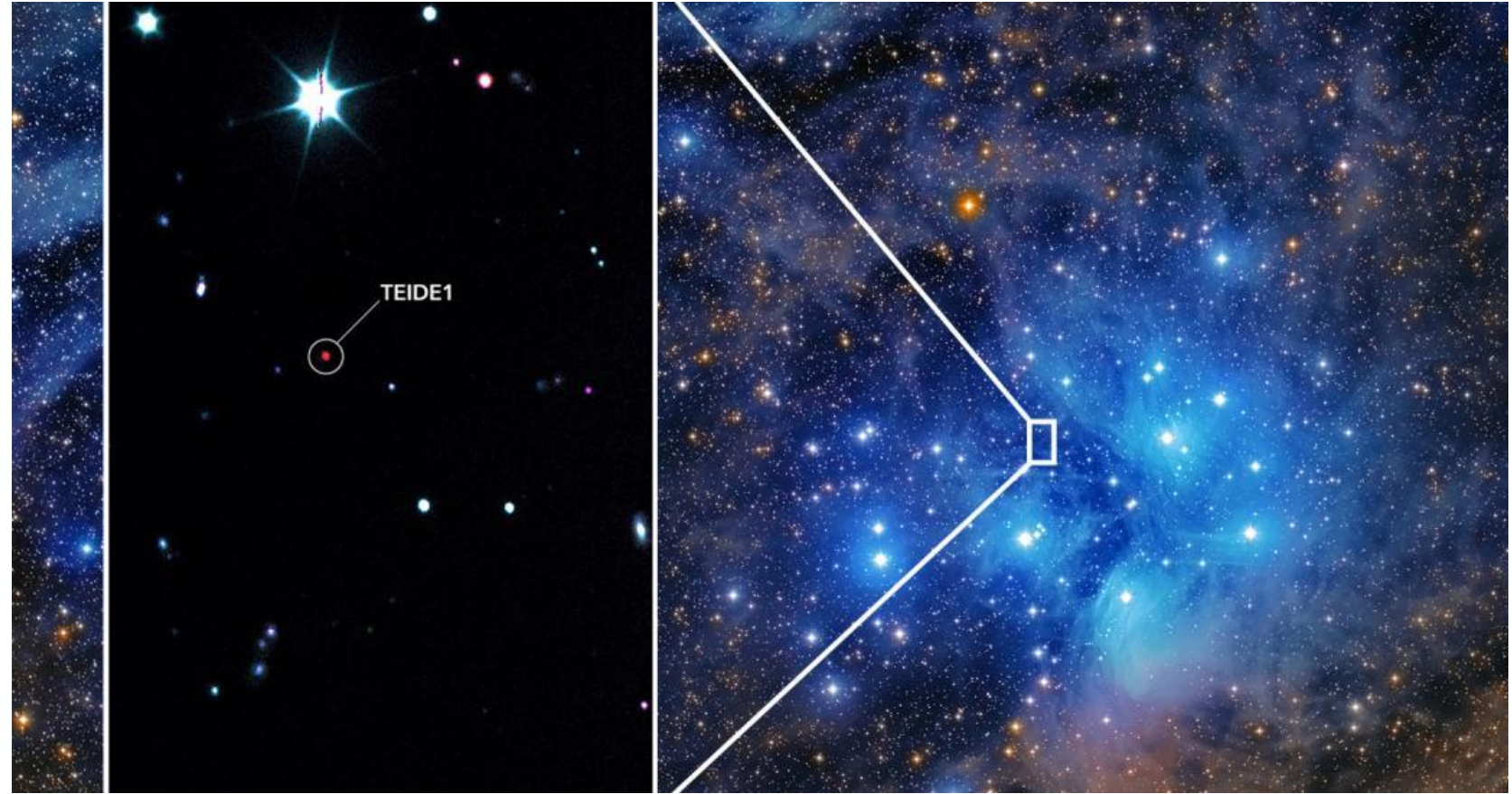
Image of the Teide 1 brown dwarf (Credit: Gran Telescopio Canarias) located in the Open Cluster of the Pleiades (Credit: Daniel López /Alfred Rosenberg, IAC)
