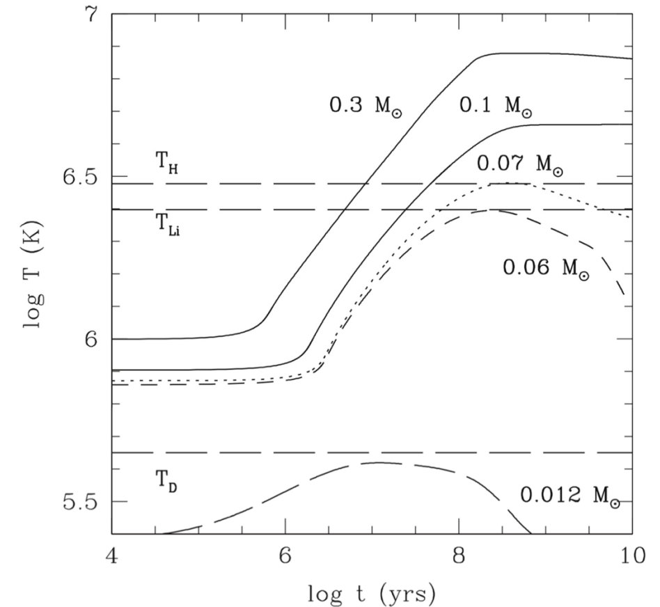
Central temperature of stars, brown dwarfs and “planetary-mass objects” as a function of age. Credits: Caballero 2018, based on Charbrier & Baraffe 2000
