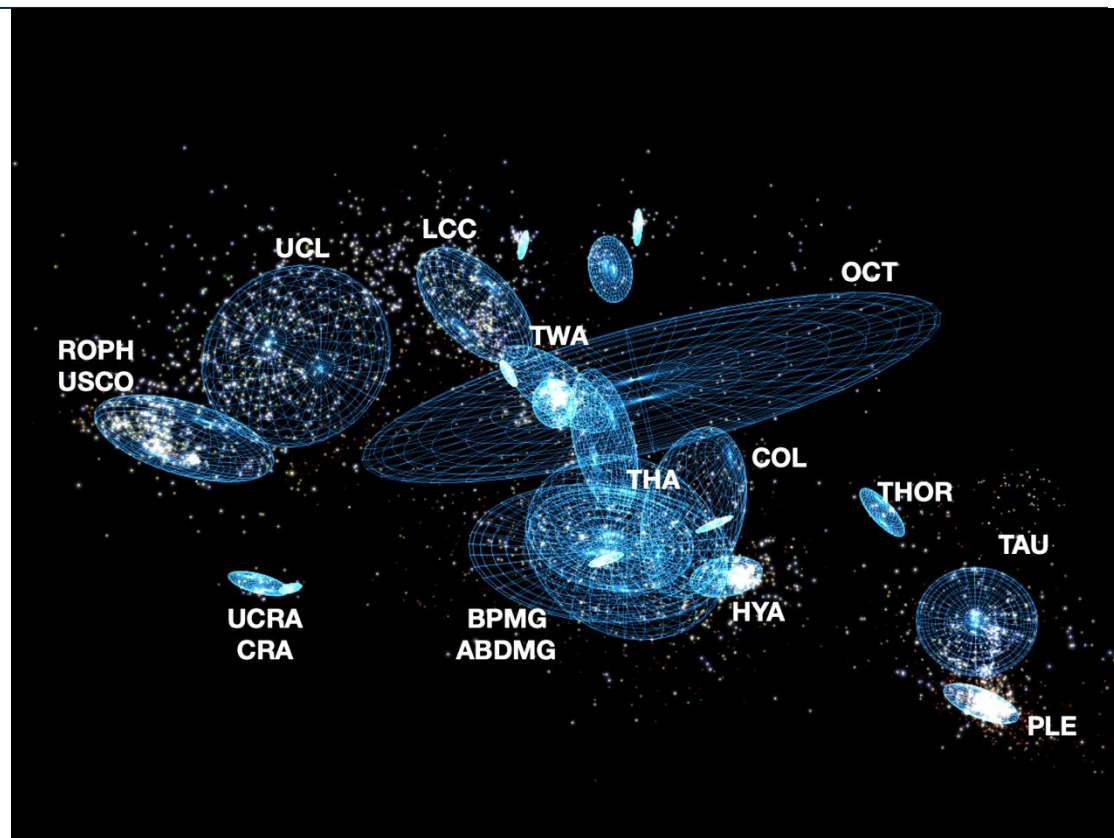
An image of the 150 pc area around the Sun highlighting the locations of star forming regions and nearby moving groups. Credits: Faherty et al. 2020
