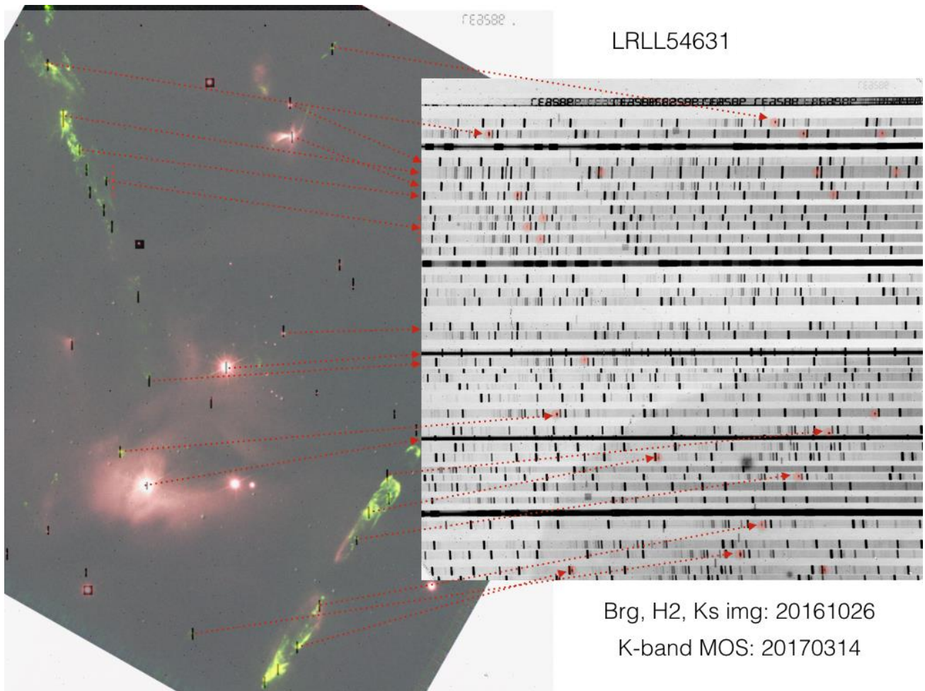
Figure 11: An example of a multi-object spectroscopic observation with LUCI ARGOS of LRL54631 showing massive H _2 jets whose spectroscopic properties can be measured in 39 individual locations with one observation. The high spatial resolution with ARGOS allows for small slits and thus enables a spectral resolution of R=10000 .
